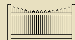
SPADE SCALLOP PICKET 2"x 6" Bottom Rail 8' wide panels available 5', 4' and 3' high
