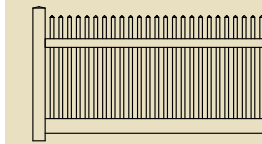
CLASSIC STRAIGHT PICKET 2"x 6" Bottom Rail 8' wide panels available 6', 5', 4' and 3' high 6' wide panel available 4' high
