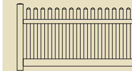
DOGEAR STRAIGHT PICKET 2"x 6" Bottom Rail 8' wide panels available 5', 4' and 3' high 6' wide panel available 4' high
