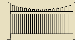
DOGEAR SCALLOP PICKET 2"x 6" Bottom Rail 8' wide panels available 5', 4' and 3' high 6' wide panel available 4' high
